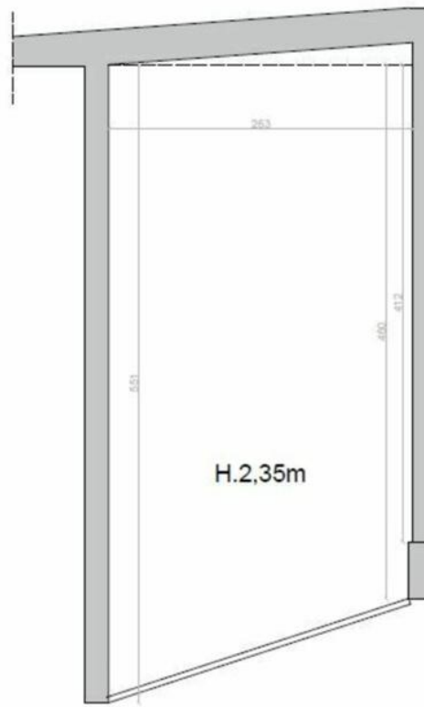
Mirabel Garage Scala 1:50
